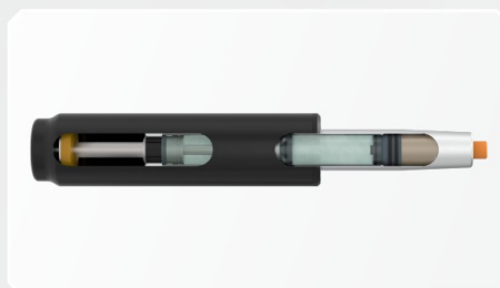
100mm Class 3 Gas Lift ensures 10cm height adjustment over 100,000 times
